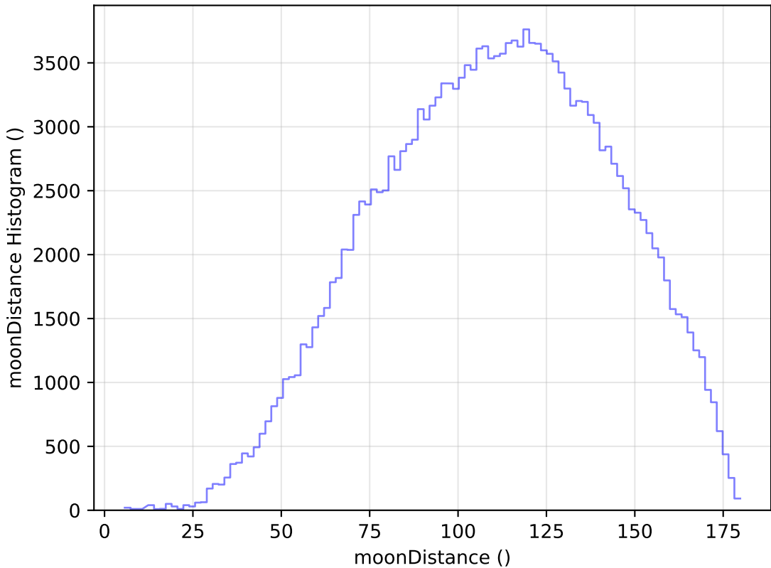
no_magell_roll_v3.4_10yrs All sky g band: moonDistance Histogram
