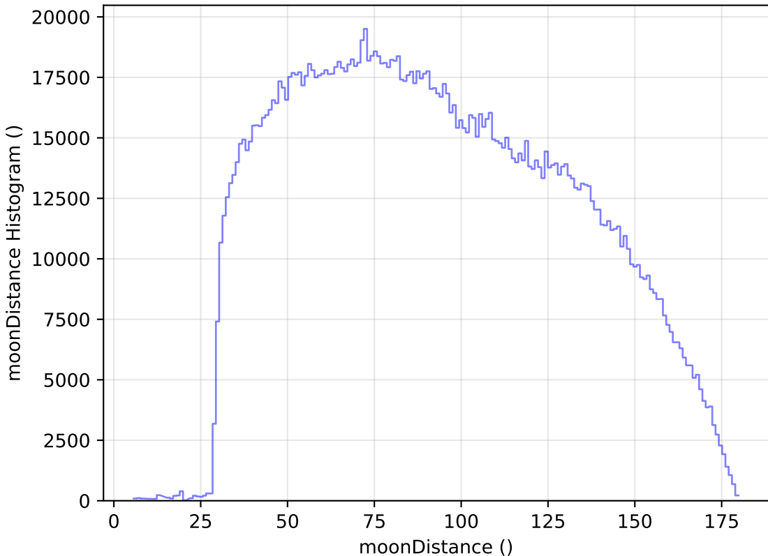
no_magell_roll_v3.4_10yrs All sky all bands: moonDistance Histogram
