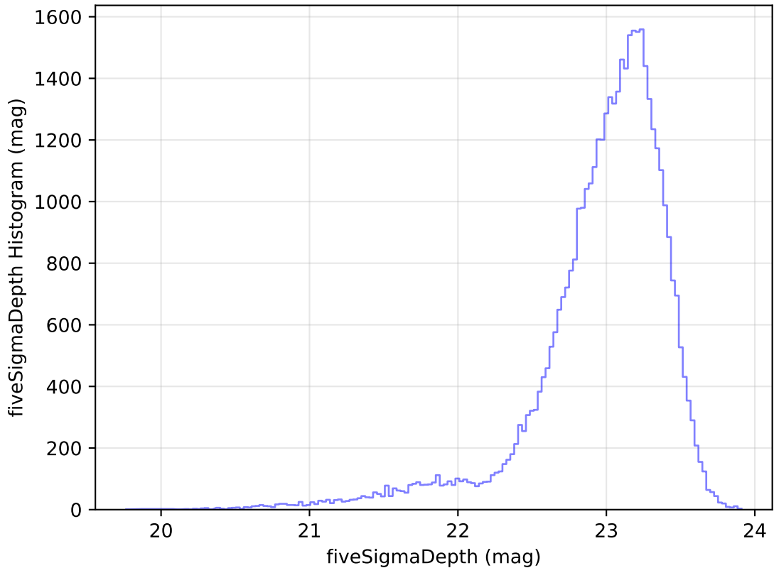
no_magell_roll_v3.4_10yrs Yr 1 z band: fiveSigmaDepth Histogram
