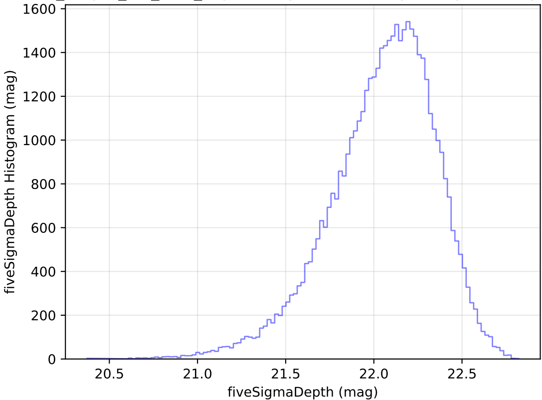
no_magell_roll_v3.4_10yrs Yr 1 y band: fiveSigmaDepth Histogram
