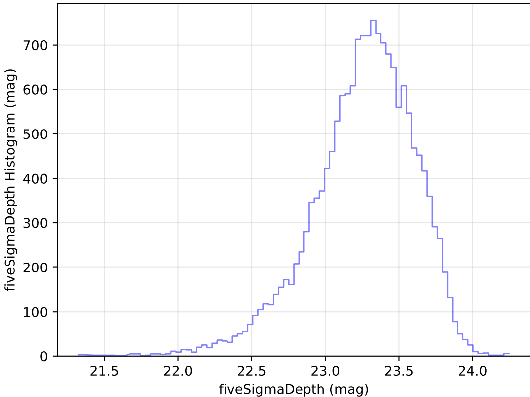
no_magell_roll_v3.4_10yrs Yr 1 u band: fiveSigmaDepth Histogram
