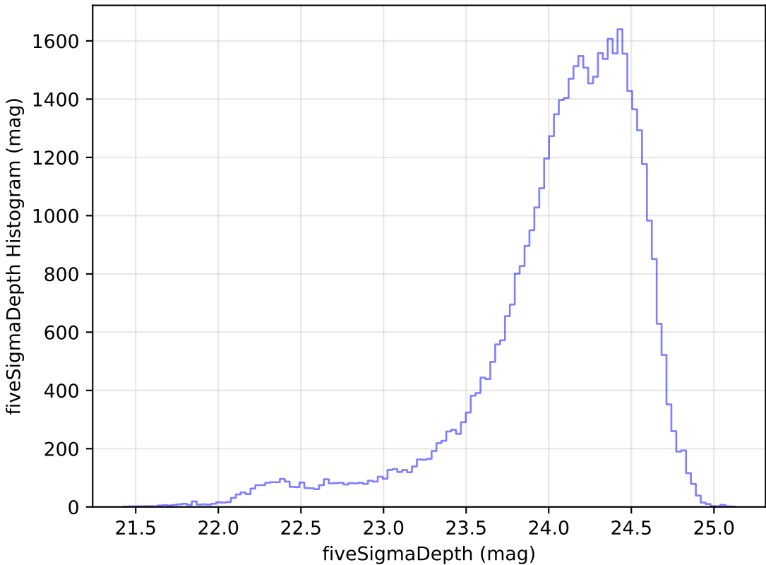
no_magell_roll_v3.4_10yrs Yr 1 r band: fiveSigmaDepth Histogram
