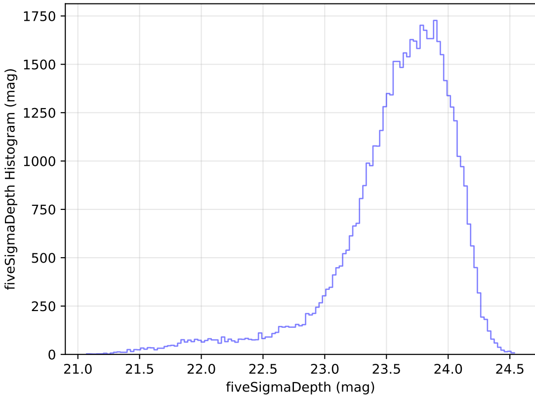
no_magell_roll_v3.4_10yrs Yr 1 i band: fiveSigmaDepth Histogram
