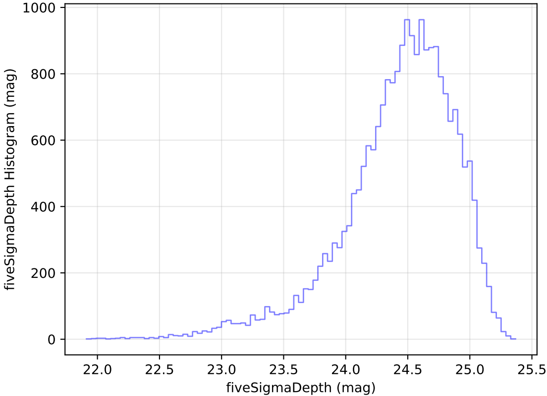
no_magell_roll_v3.4_10yrs Yr 1 g band: fiveSigmaDepth Histogram
