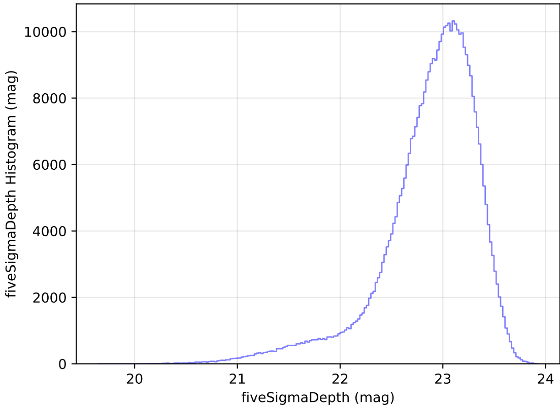
no_magell_roll_v3.4_10yrs WFD z band: fiveSigmaDepth Histogram
