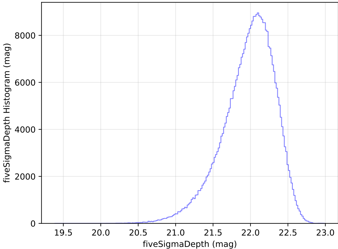
no_magell_roll_v3.4_10yrs WFD y band: fiveSigmaDepth Histogram
