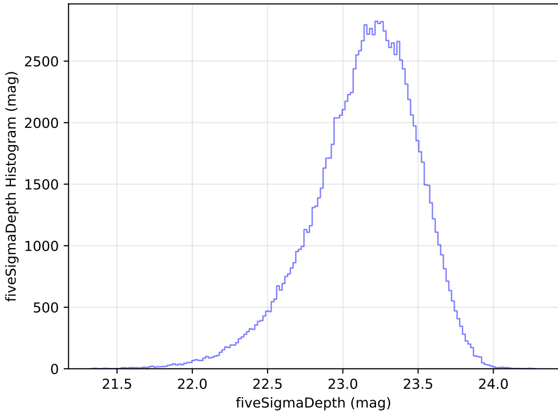
no_magell_roll_v3.4_10yrs WFD u band: fiveSigmaDepth Histogram
