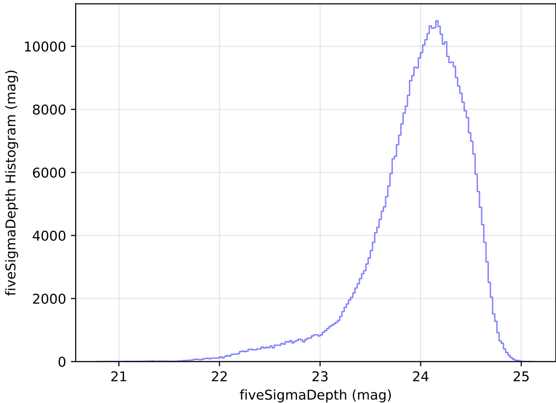
no_magell_roll_v3.4_10yrs WFD r band: fiveSigmaDepth Histogram
