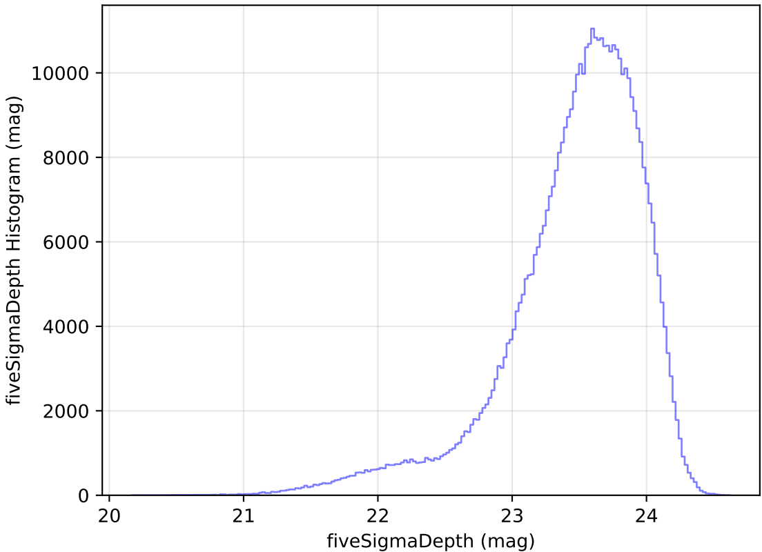
no_magell_roll_v3.4_10yrs WFD i band: fiveSigmaDepth Histogram
