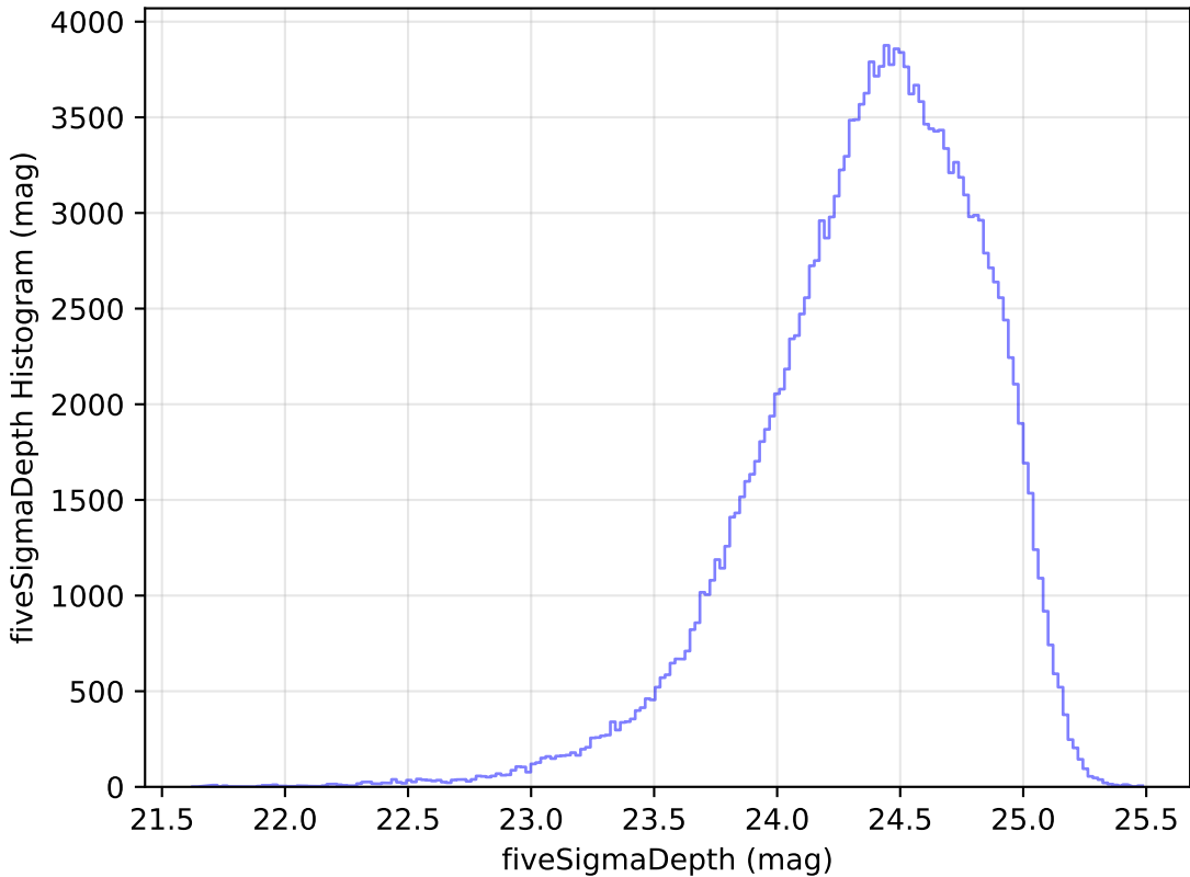
no_magell_roll_v3.4_10yrs WFD g band: fiveSigmaDepth Histogram
