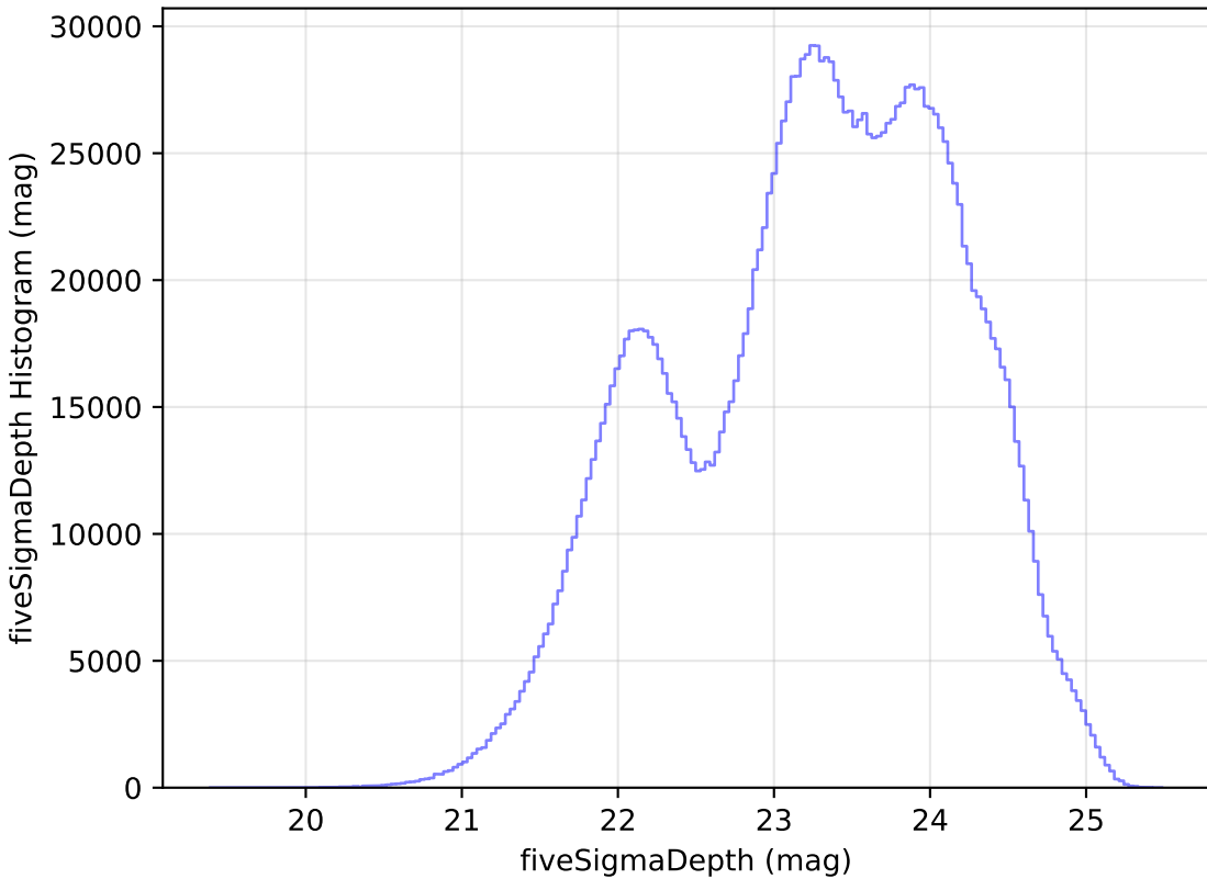
no_magell_roll_v3.4_10yrs WFD all bands: fiveSigmaDepth Histogram
