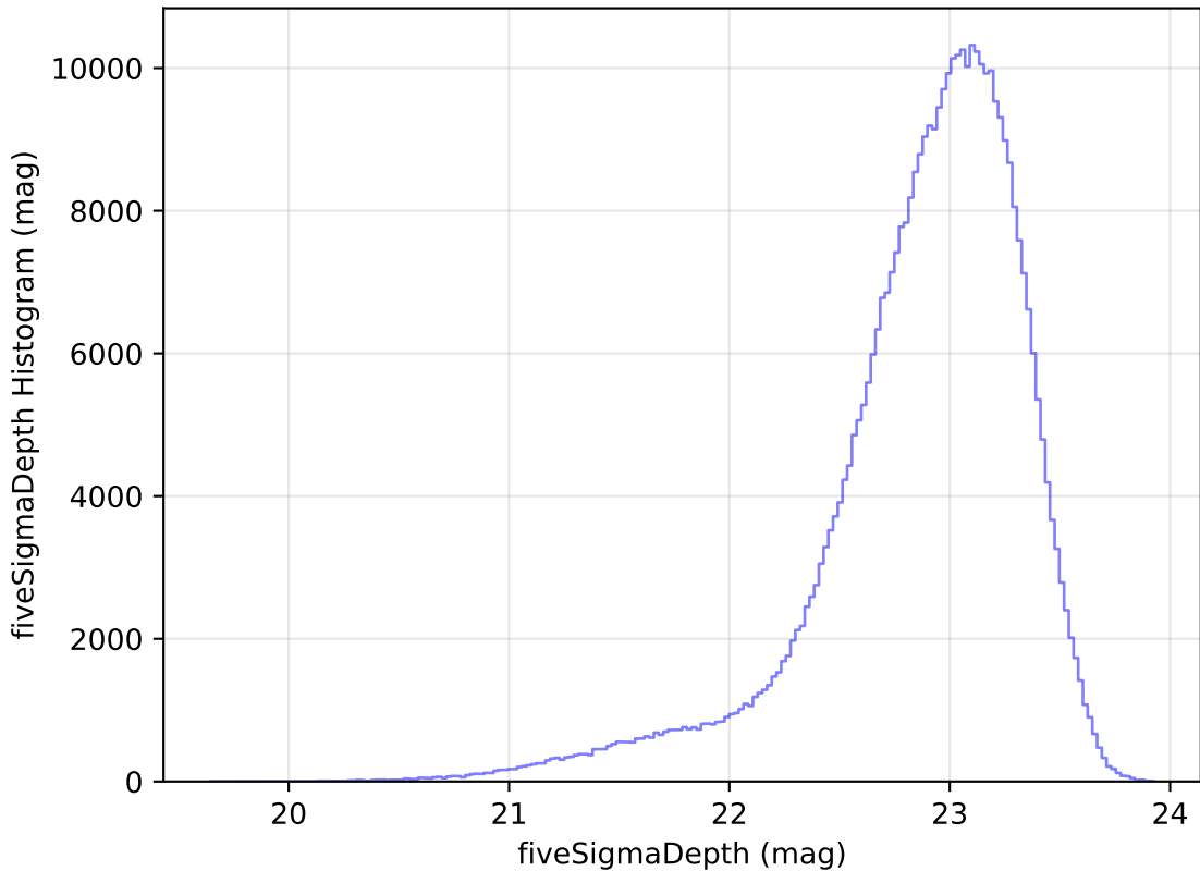
no_magell_roll_v3.4_10yrs All sky z band: fiveSigmaDepth Histogram
