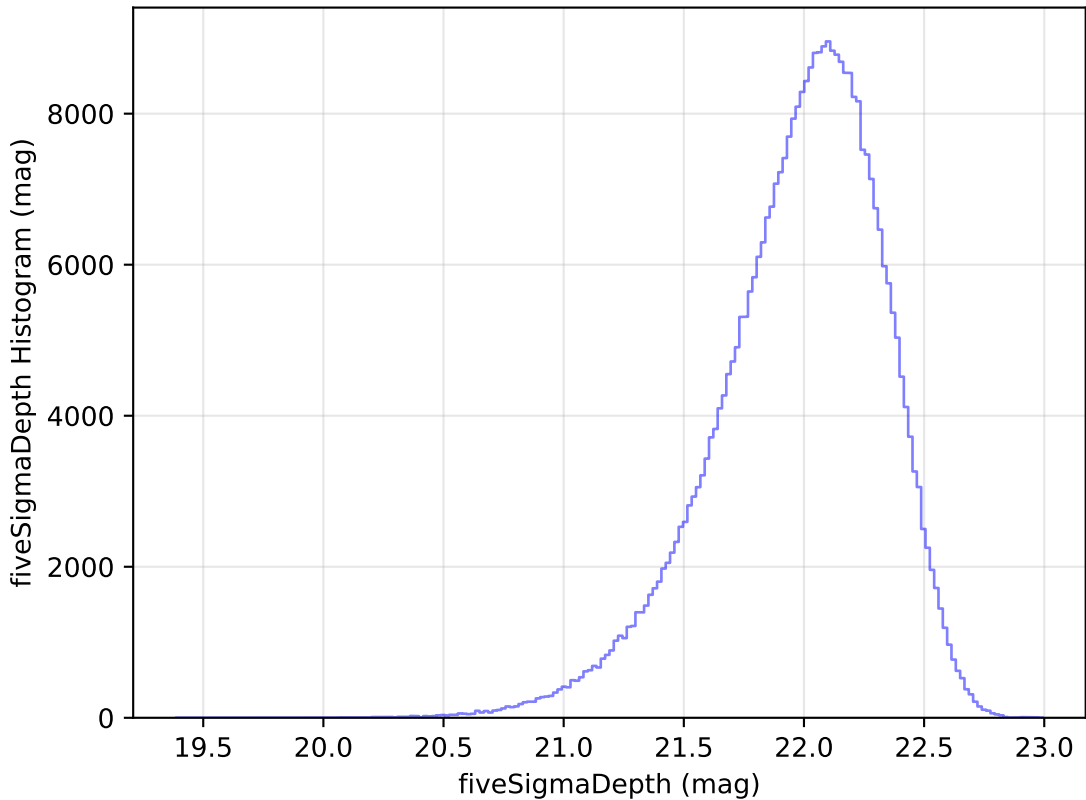
no_magell_roll_v3.4_10yrs All sky y band: fiveSigmaDepth Histogram
