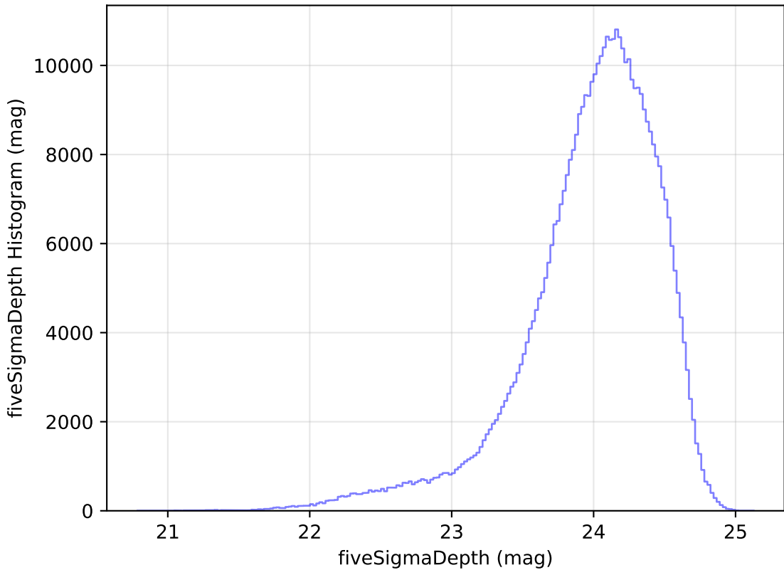
no_magell_roll_v3.4_10yrs All sky r band: fiveSigmaDepth Histogram
