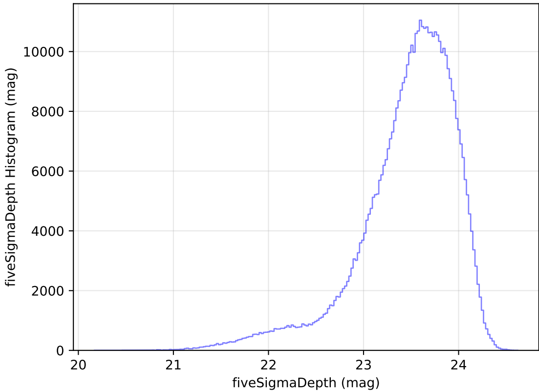
no_magell_roll_v3.4_10yrs All sky i band: fiveSigmaDepth Histogram
