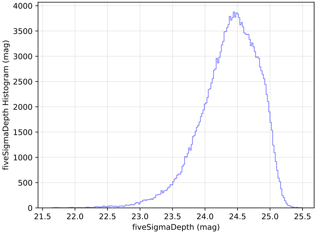
no_magell_roll_v3.4_10yrs All sky g band: fiveSigmaDepth Histogram
