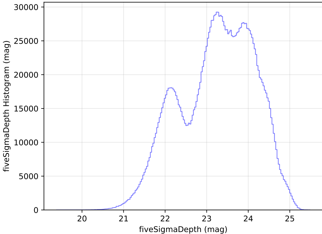
no_magell_roll_v3.4_10yrs All sky all bands: fiveSigmaDepth Histogram
