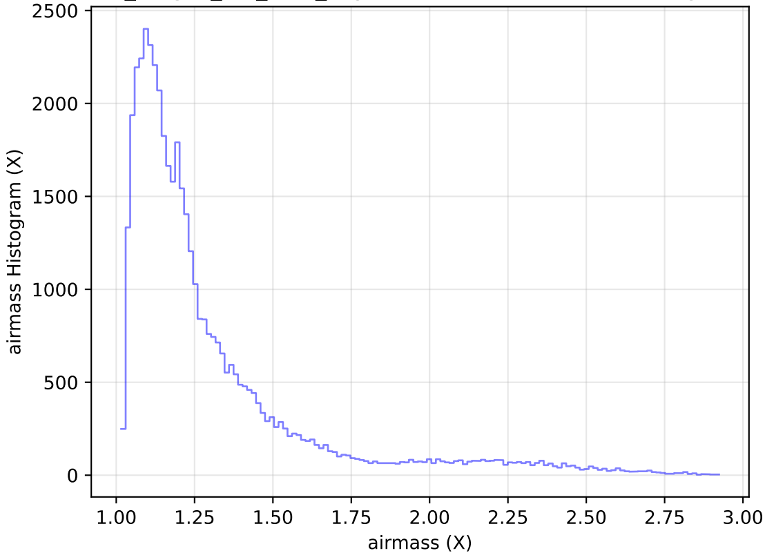
no_magell_roll_v3.4_10yrs Yr 1 z band: airmass Histogram
