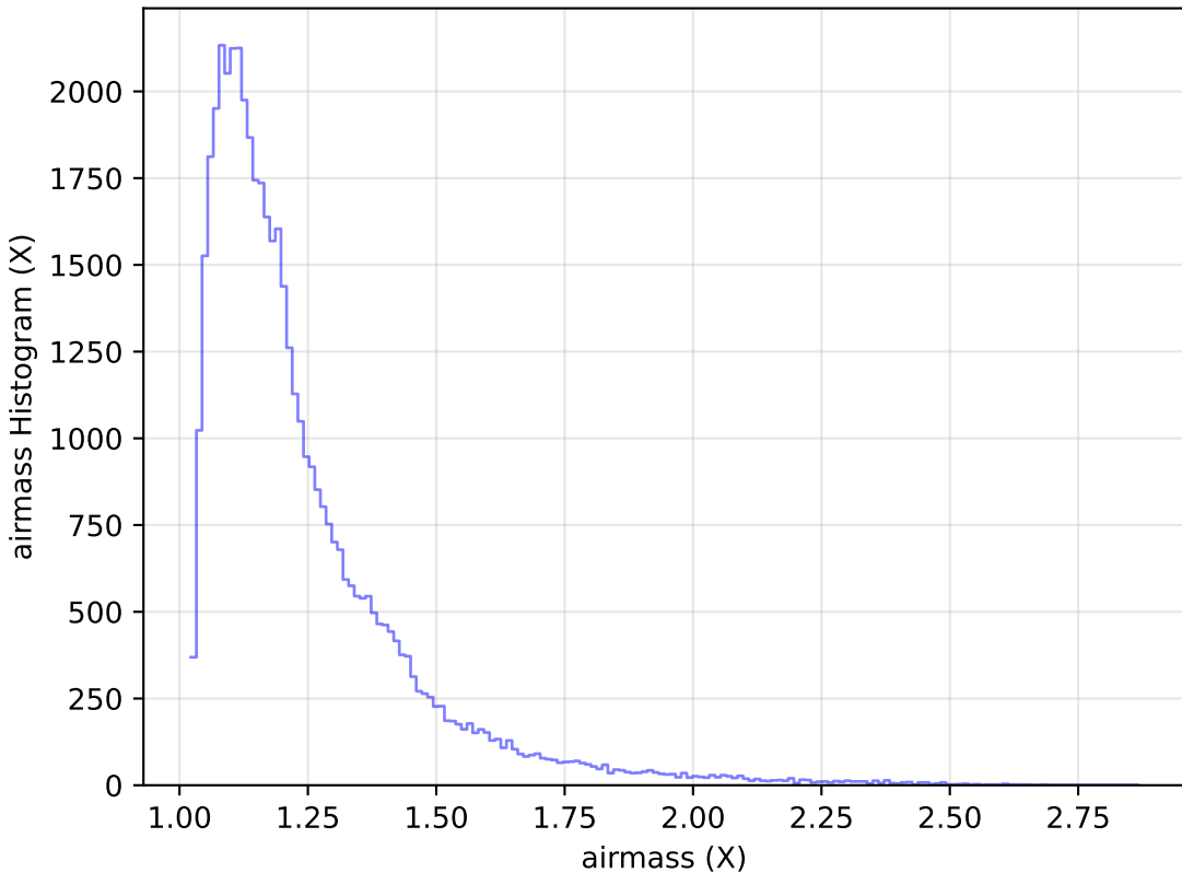
no_magell_roll_v3.4_10yrs Yr 1 y band: airmass Histogram
