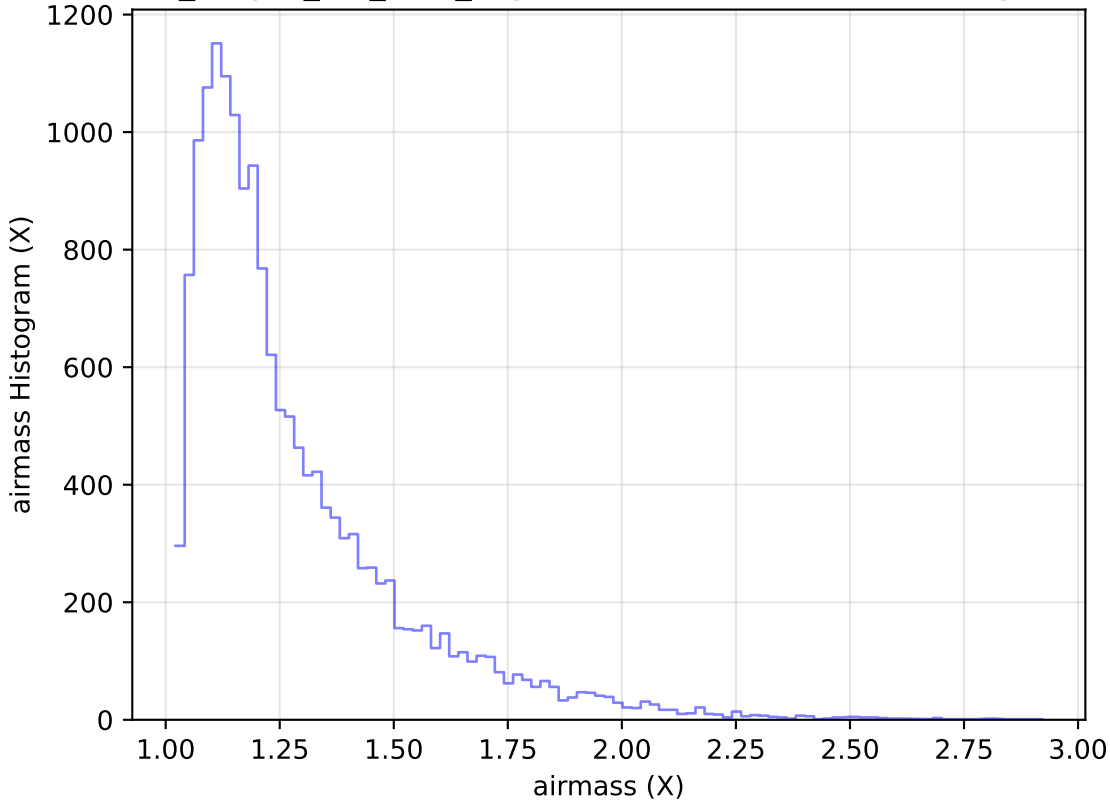
no_magell_roll_v3.4_10yrs Yr 1 u band: airmass Histogram
