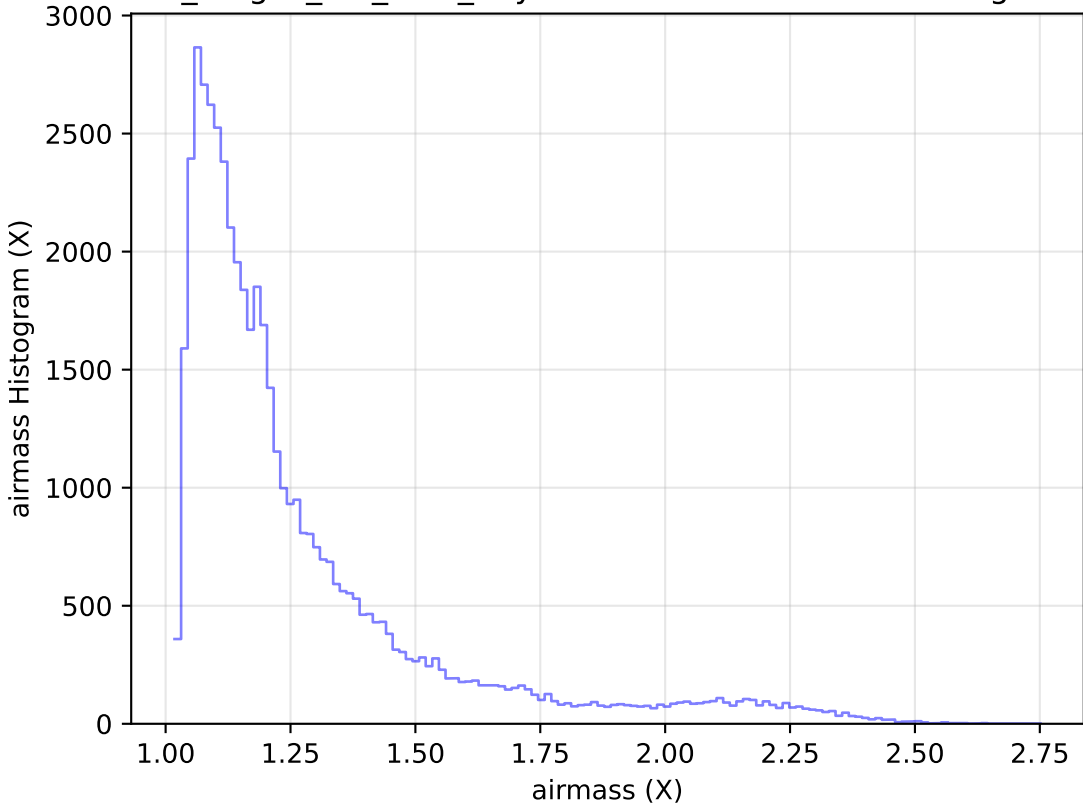
no_magell_roll_v3.4_10yrs Yr 1 r band: airmass Histogram
