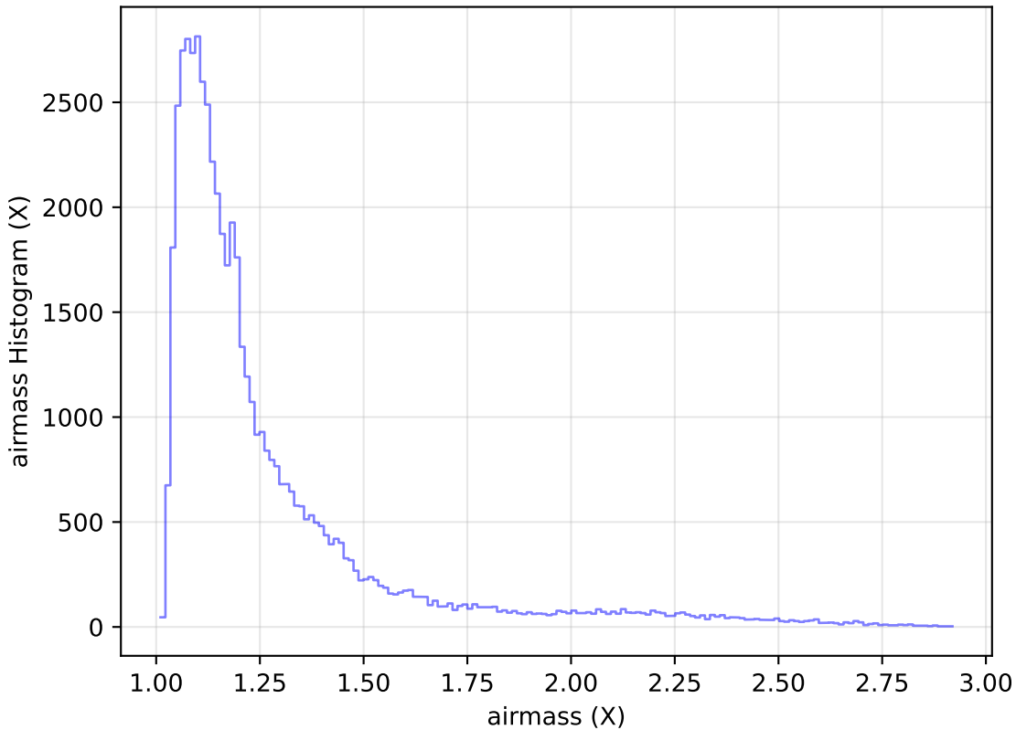
no_magell_roll_v3.4_10yrs Yr 1 i band: airmass Histogram
