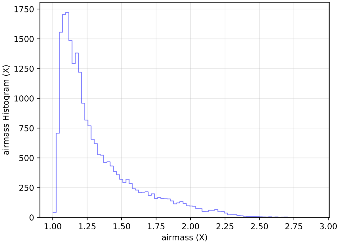
no_magell_roll_v3.4_10yrs Yr 1 g band: airmass Histogram
