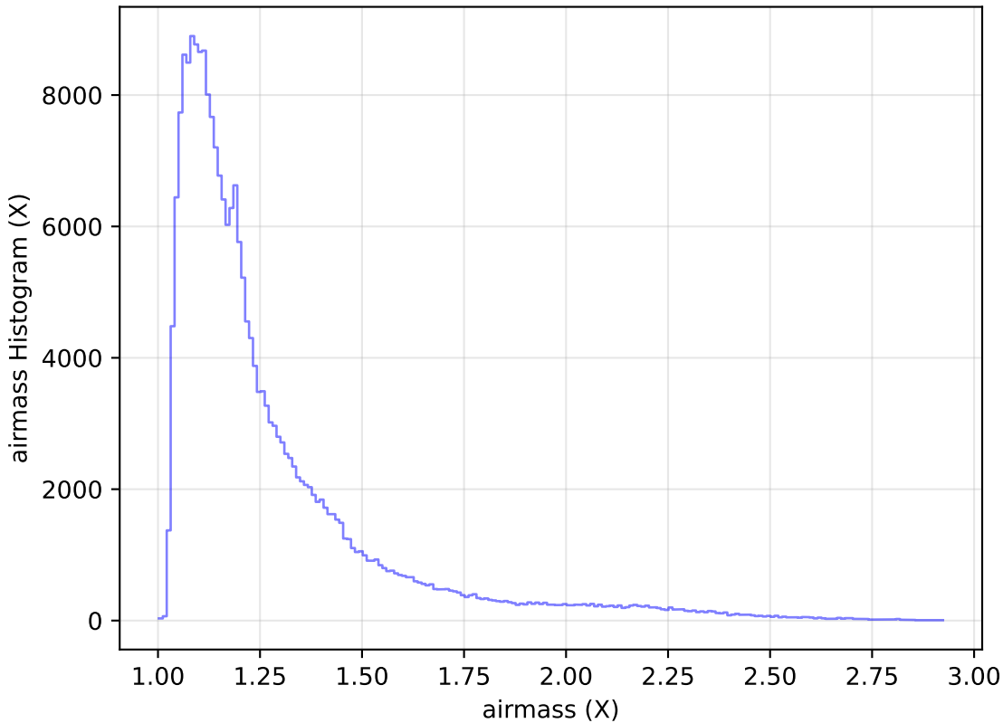
no_magell_roll_v3.4_10yrs Yr 1 all bands: airmass Histogram
