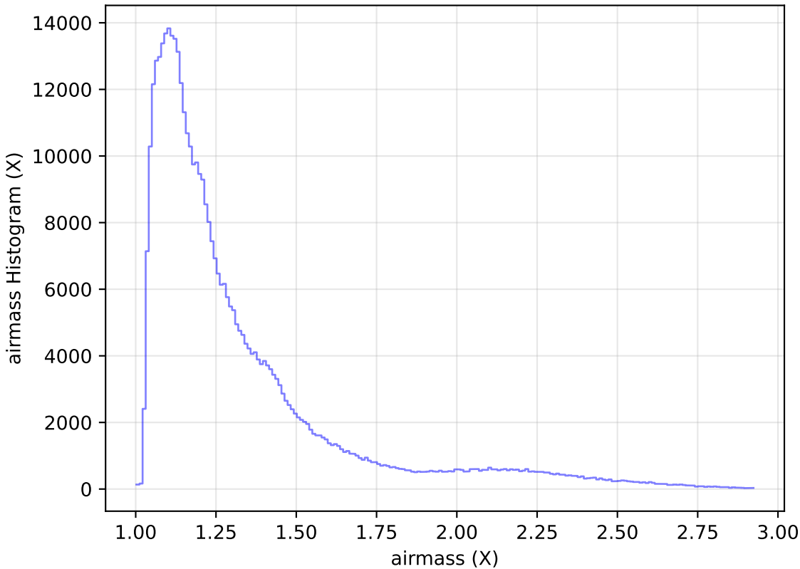
no_magell_roll_v3.4_10yrs WFD z band: airmass Histogram
