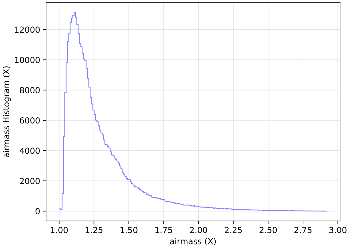
no_magell_roll_v3.4_10yrs WFD y band: airmass Histogram
