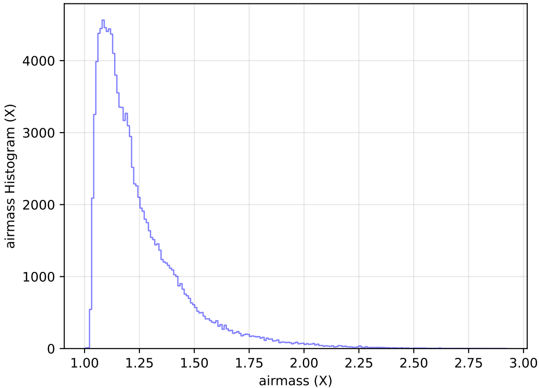
no_magell_roll_v3.4_10yrs WFD u band: airmass Histogram
