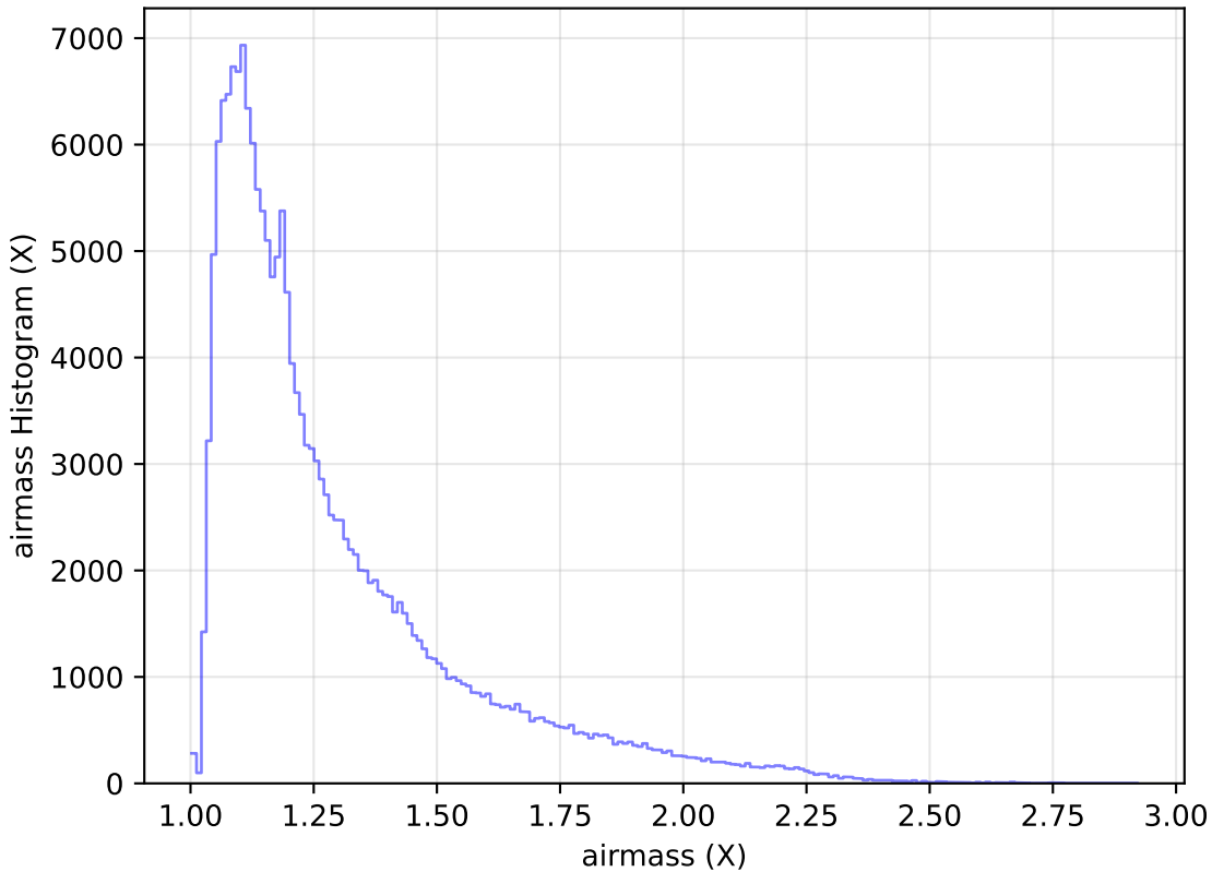
no_magell_roll_v3.4_10yrs WFD g band: airmass Histogram
