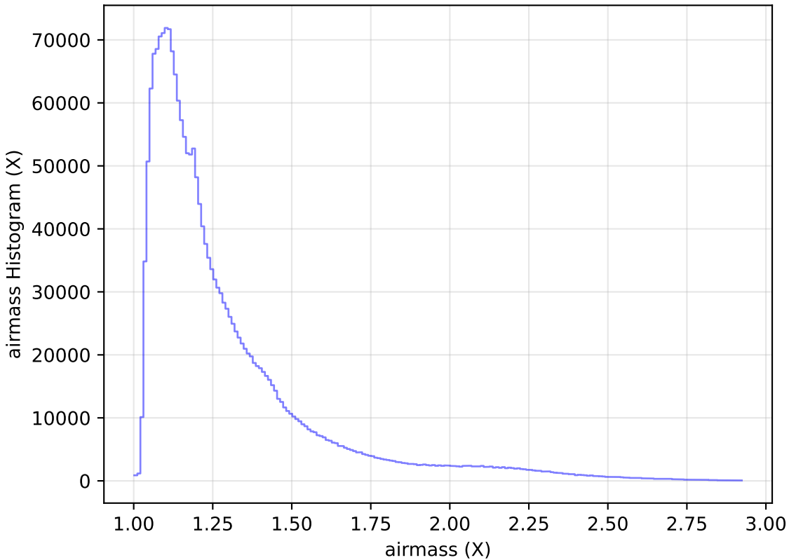
no_magell_roll_v3.4_10yrs WFD all bands: airmass Histogram
