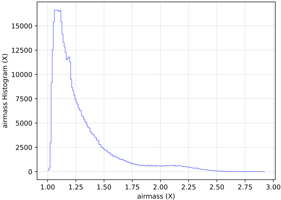
no_magell_roll_v3.4_10yrs All sky r band: airmass Histogram
