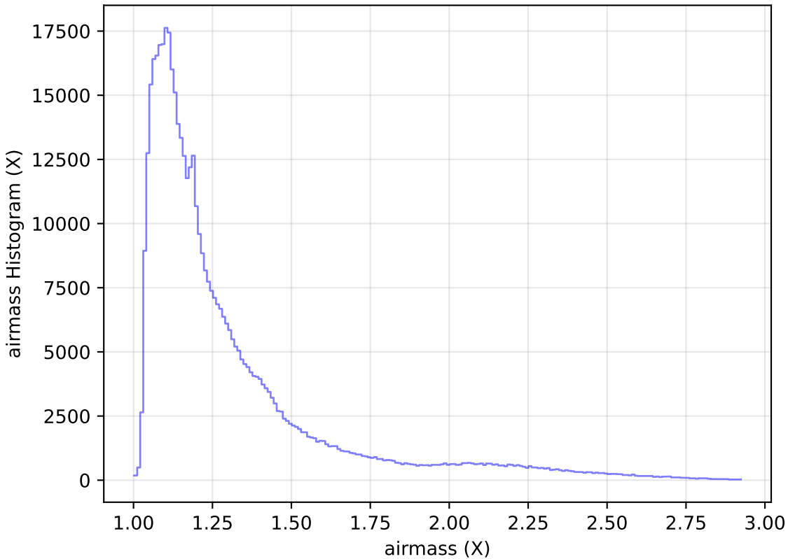
no_magell_roll_v3.4_10yrs All sky i band: airmass Histogram
