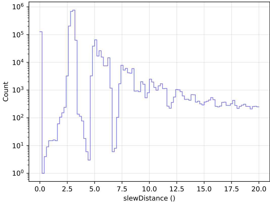
no_magell_roll_v3.4_10yrs All visits: Zoom Slew Distance Histogram
