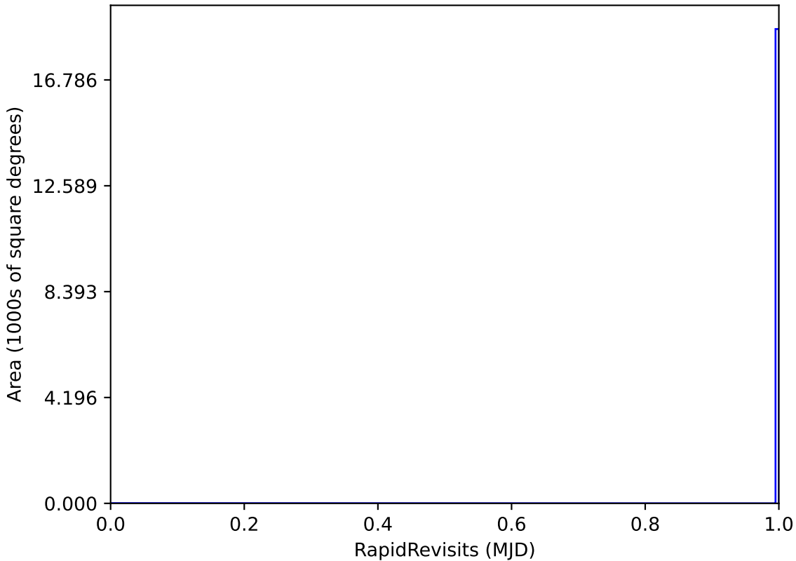
no_magell_roll_v3.4_10yrs WFD: RapidRevisits
