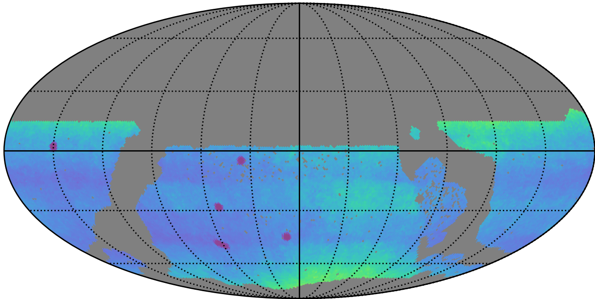
no_magell_roll_v3.4_10yrs WFD: Proper Motion Uncert @ 24.0
