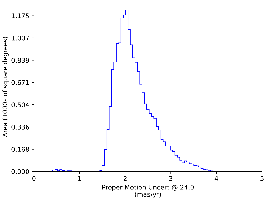
no_magell_roll_v3.4_10yrs WFD: Proper Motion Uncert @ 24.0
