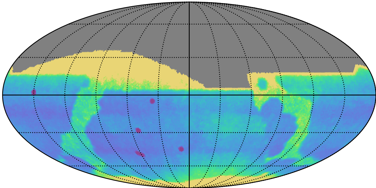
no_magell_roll_v3.4_10yrs All sky: Proper Motion Uncert @ 24.0
