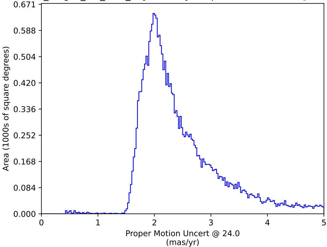
no_magell_roll_v3.4_10yrs All sky: Proper Motion Uncert @ 24.0
