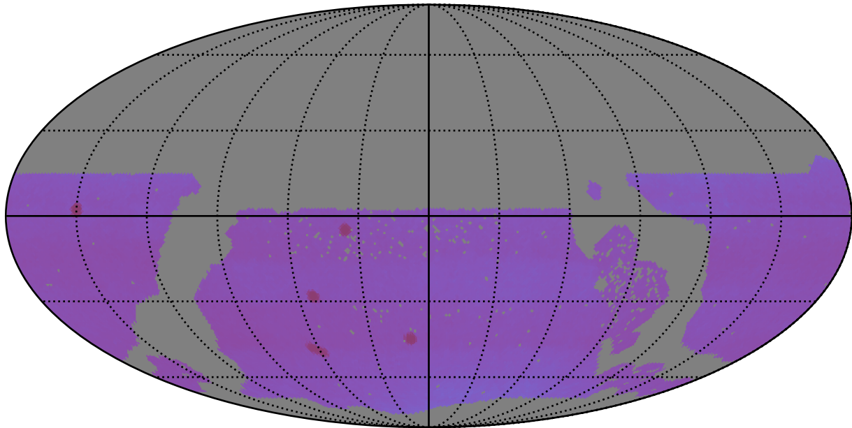
no_magell_roll_v3.4_10yrs WFD: Proper Motion Uncert @ 20.5
