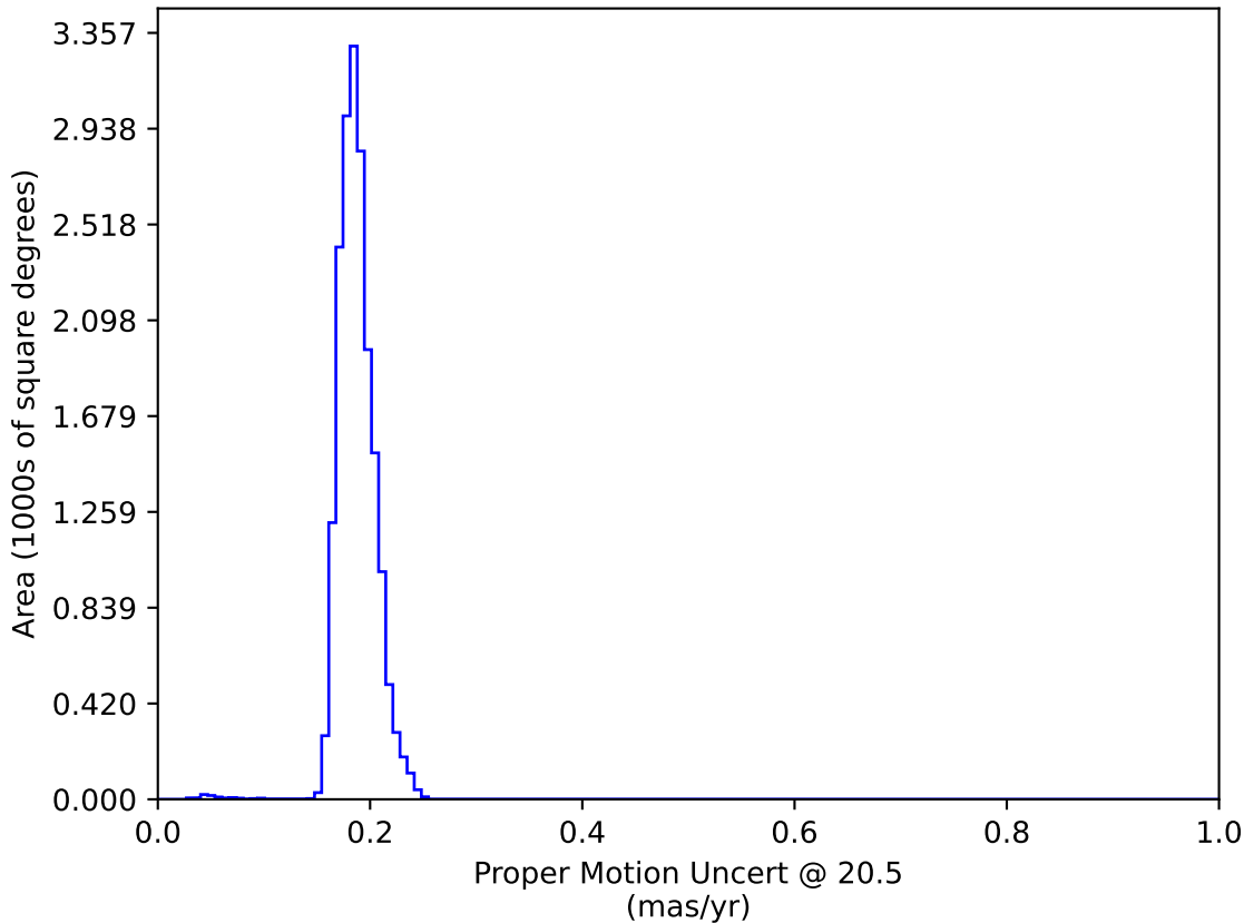
no_magell_roll_v3.4_10yrs WFD: Proper Motion Uncert @ 20.5
