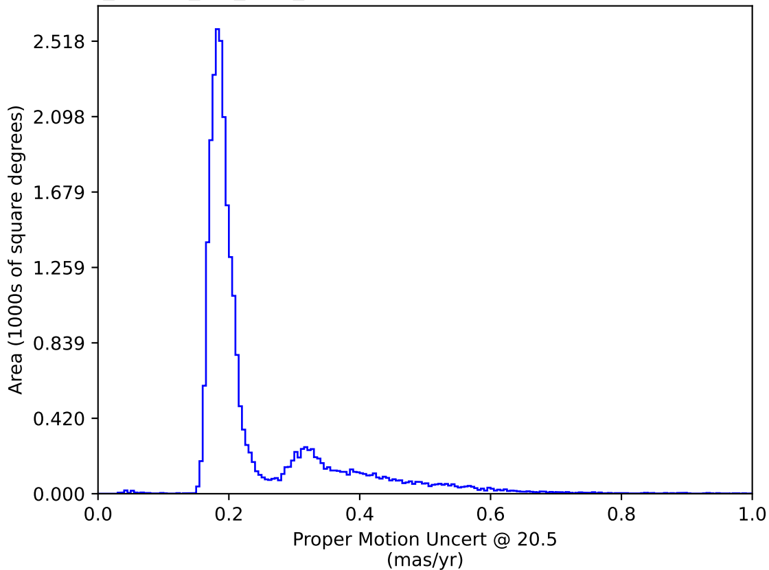
no_magell_roll_v3.4_10yrs All sky: Proper Motion Uncert @ 20.5
