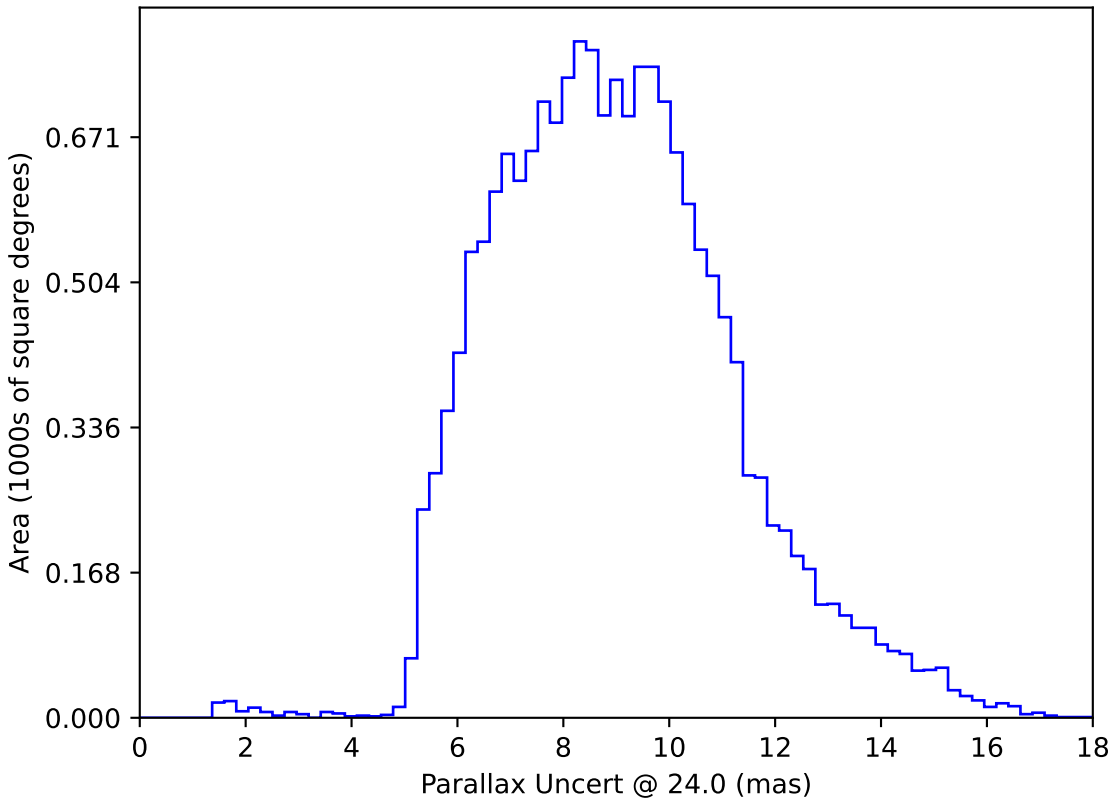
no_magell_roll_v3.4_10yrs WFD: Parallax Uncert @ 24.0
