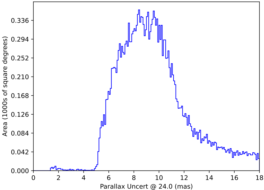
no_magell_roll_v3.4_10yrs All sky: Parallax Uncert @ 24.0
