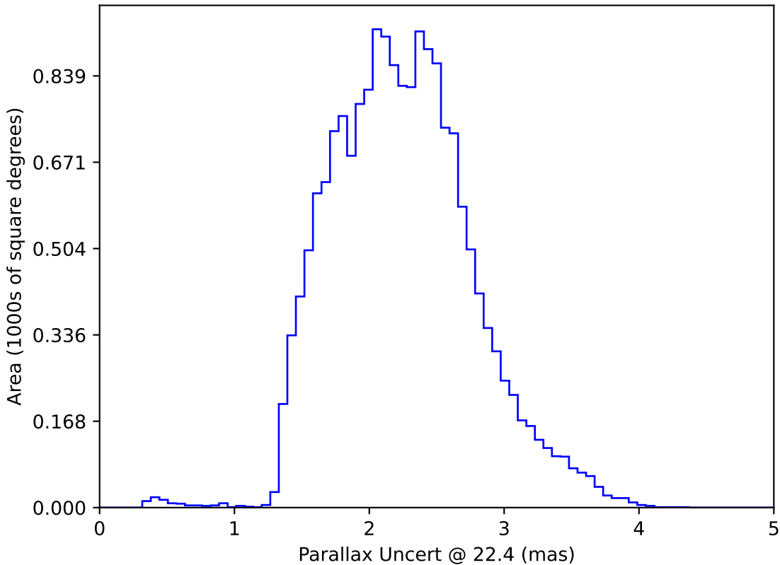
no_magell_roll_v3.4_10yrs WFD: Parallax Uncert @ 22.4
