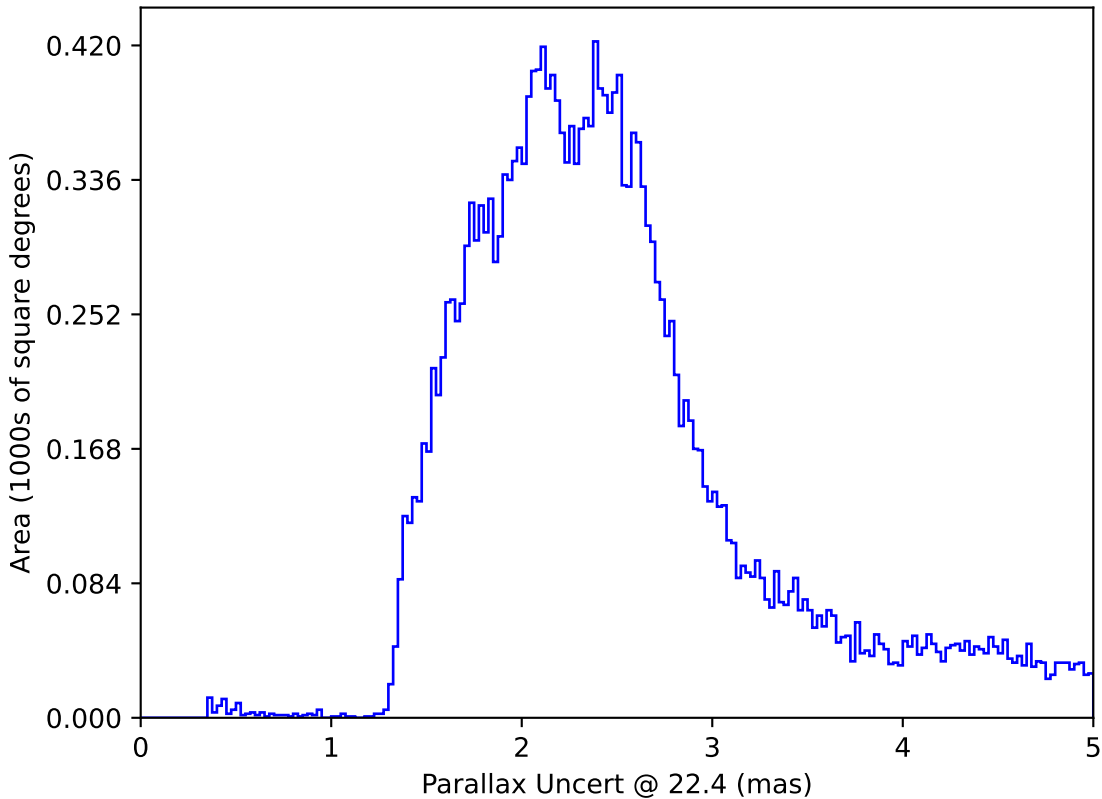
no_magell_roll_v3.4_10yrs All sky: Parallax Uncert @ 22.4
