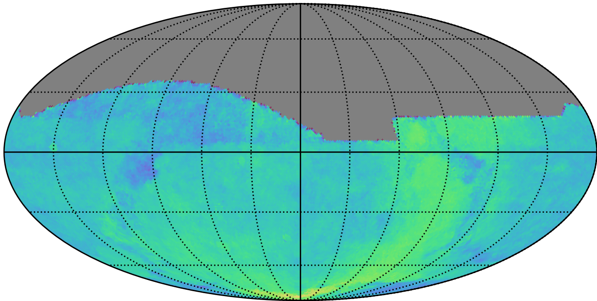
no_magell_roll_v3.4_10yrs All sky: Parallax Coverage @ 24.0
