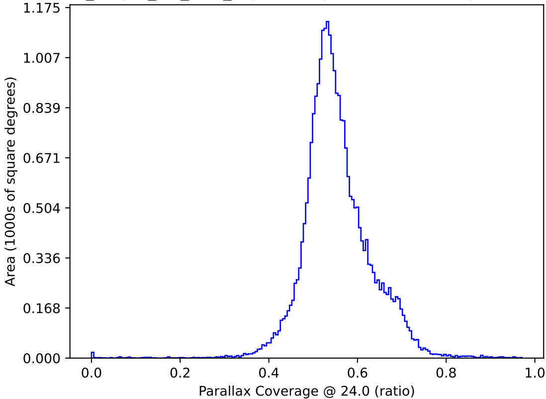
no_magell_roll_v3.4_10yrs All sky: Parallax Coverage @ 24.0
